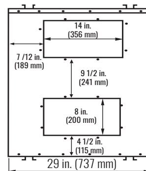
Inlet Side
